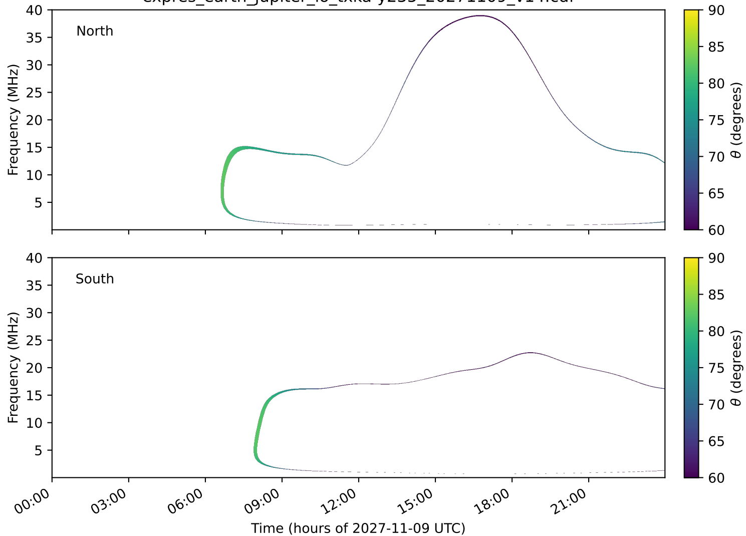
expres_earth_jupiter_io_txka-y235_20271109_v14.cdf
