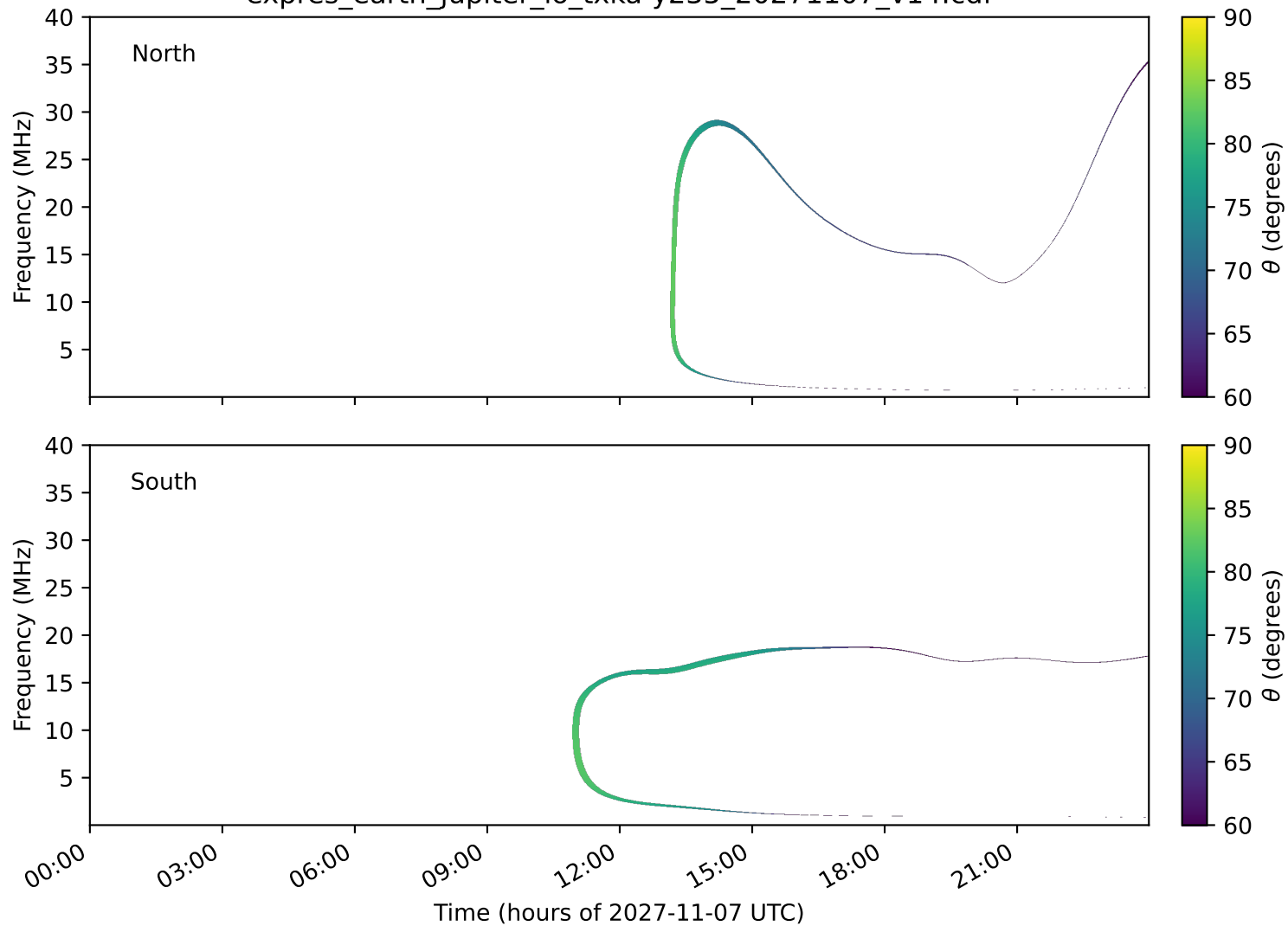
expres_earth_jupiter_io_txka-y235_20271107_v14.cdf
