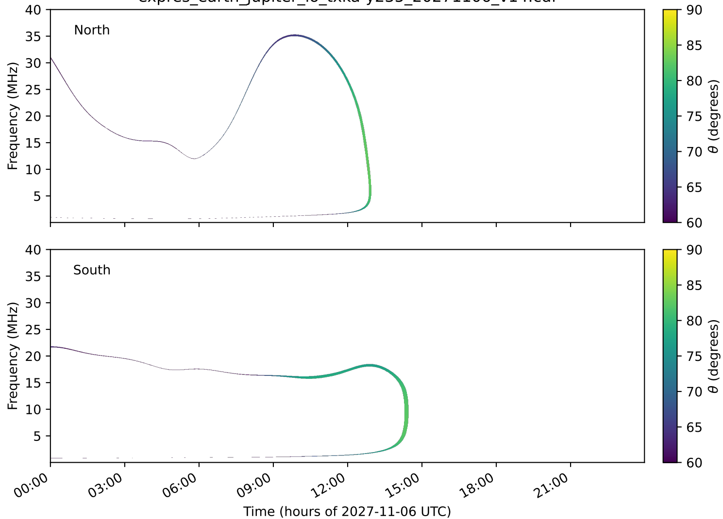
expres_earth_jupiter_io_txka-y235_20271106_v14.cdf
