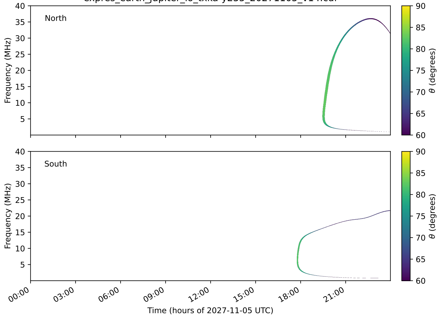
expres_earth_jupiter_io_txka-y235_20271105_v14.cdf
