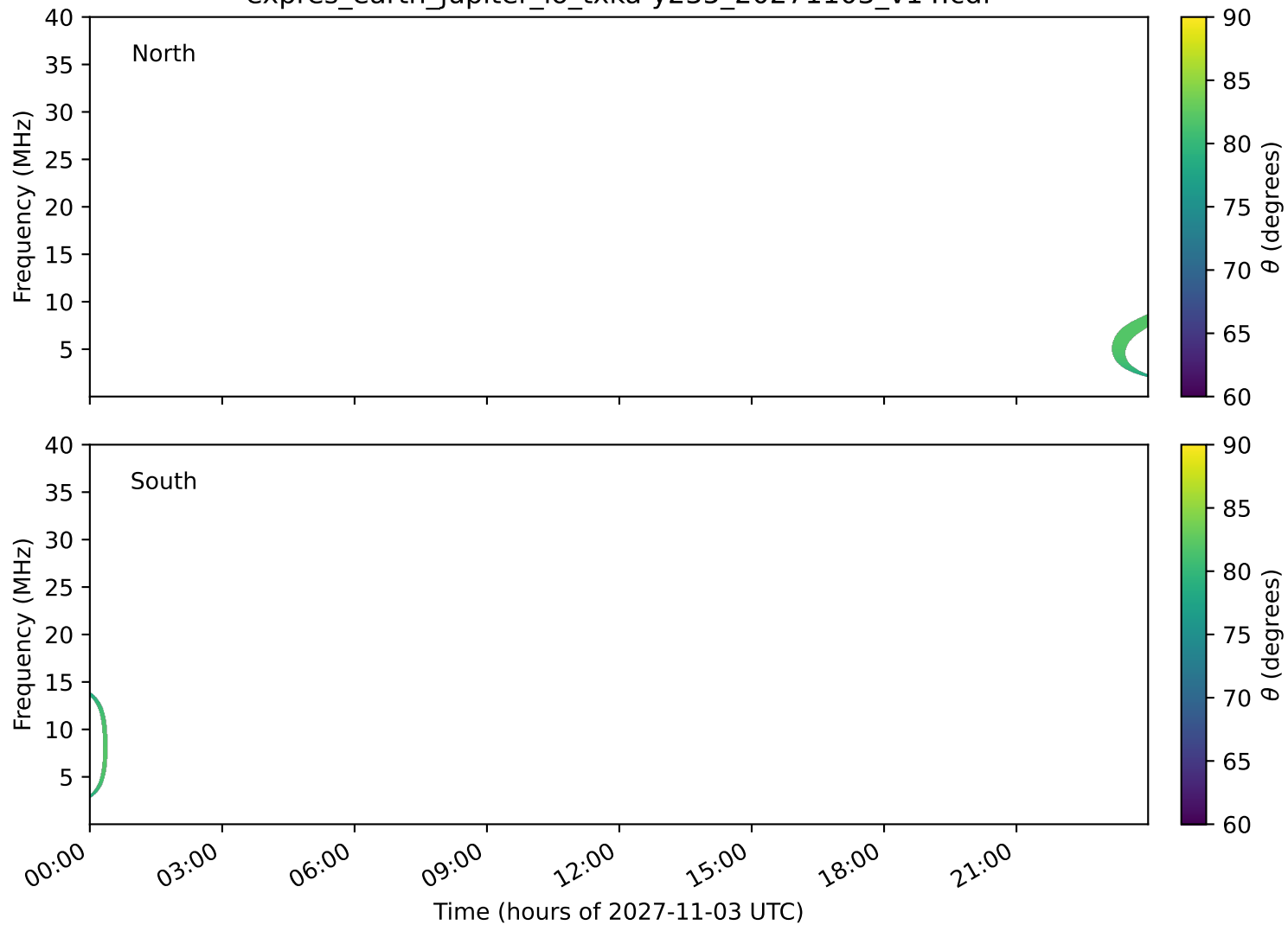
expres_earth_jupiter_io_txka-y235_20271103_v14.cdf
