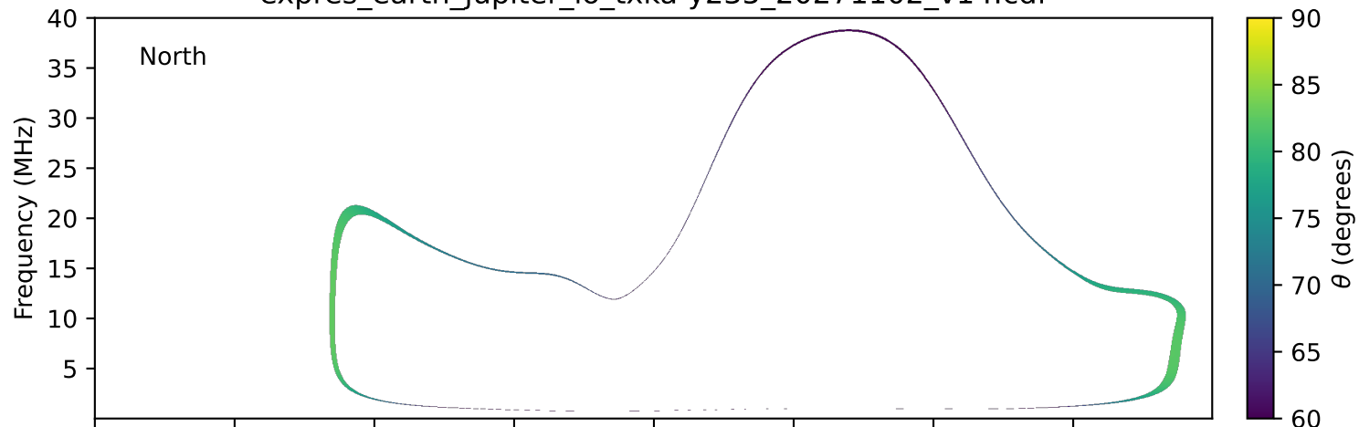
expres_earth_jupiter_io_txka-y235_20271102_v14.cdf
