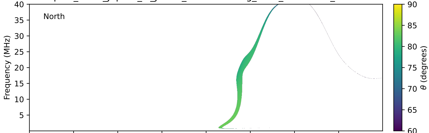
expres_earth_jupiter_io_jrm33_lossc-wid1deg_3kev_20271130_v11.cdf
