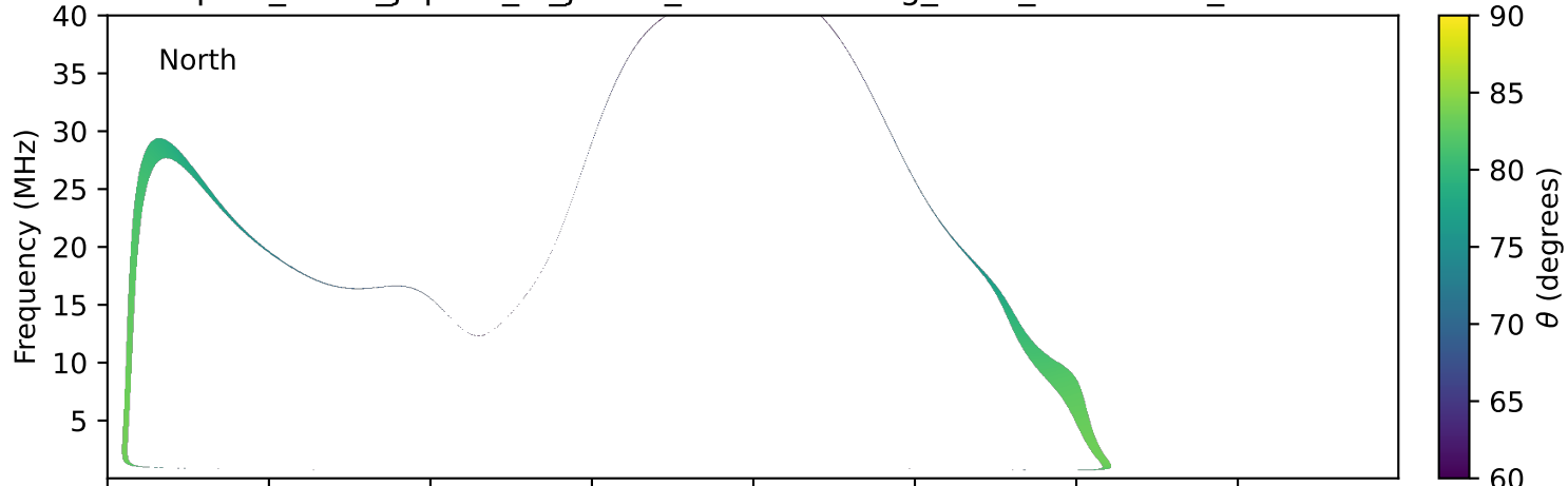
expres_earth_jupiter_io_jrm33_lossc-wid1deg_3kev_20271127_v11.cdf
