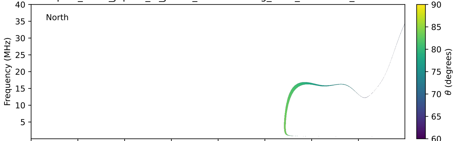
expres_earth_jupiter_io_jrm33_lossc-wid1deg_3kev_20271121_v11.cdf
