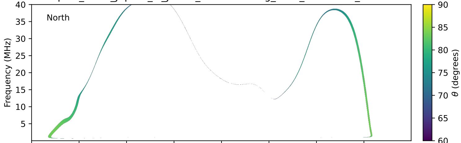
expres_earth_jupiter_io_jrm33_lossc-wid1deg_3kev_20271111_v11.cdf
