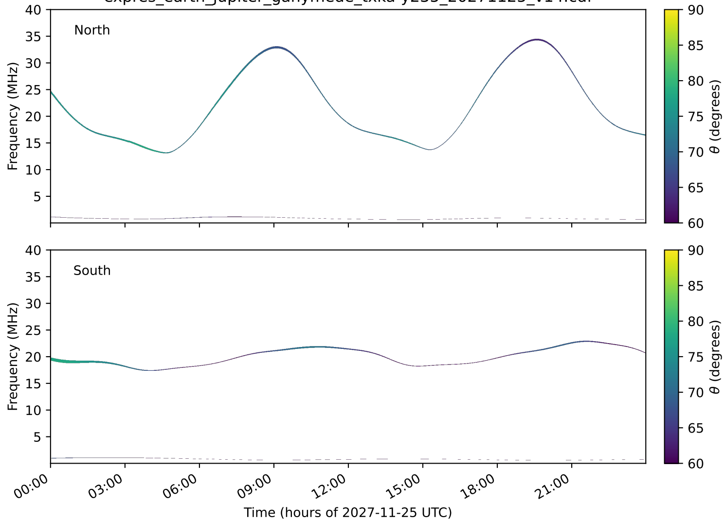
expres_earth_jupiter_ganymede_txka-y235_20271125_v14.cdf
