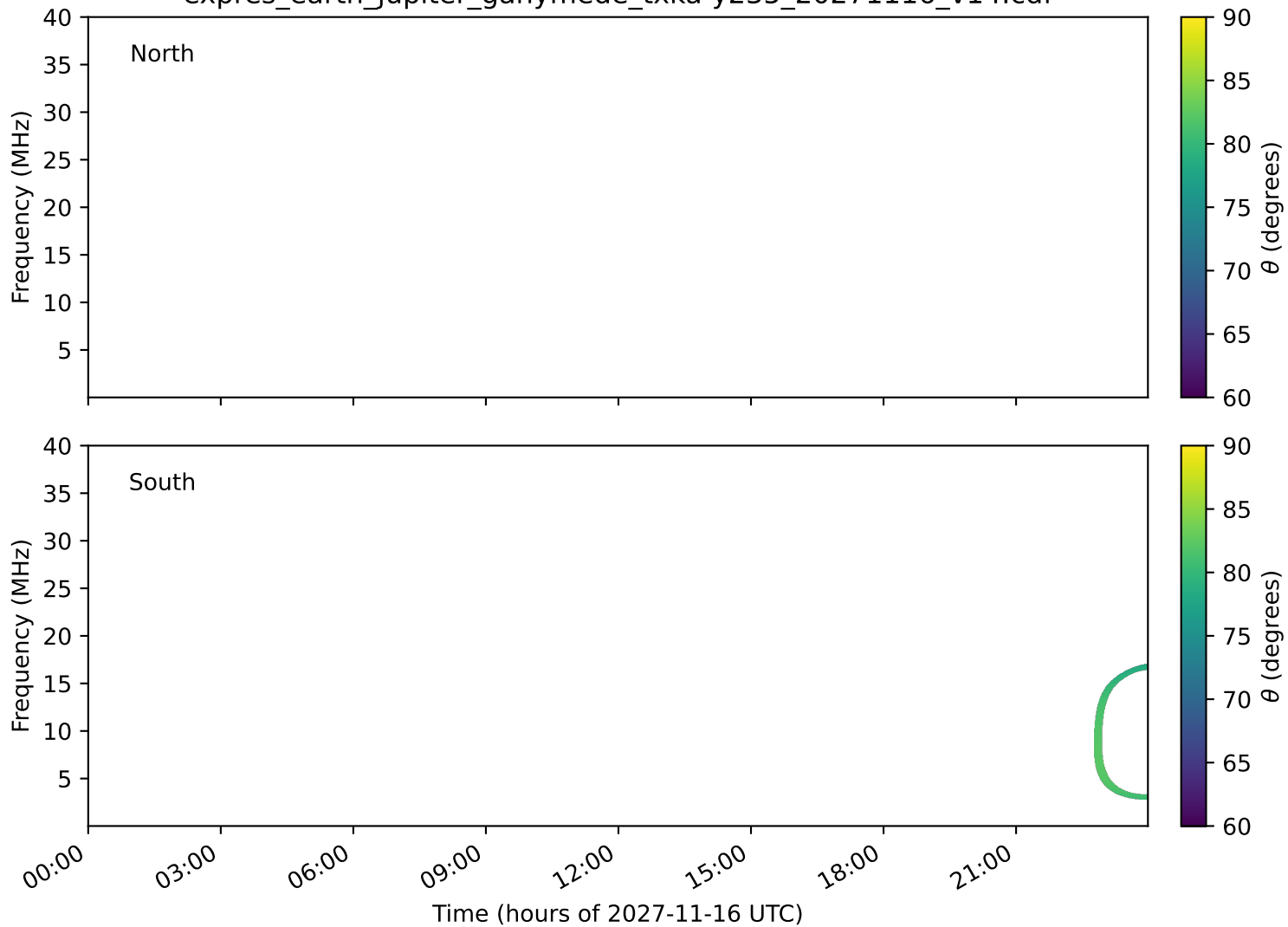
expres_earth_jupiter_ganymede_txka-y235_20271116_v14.cdf
