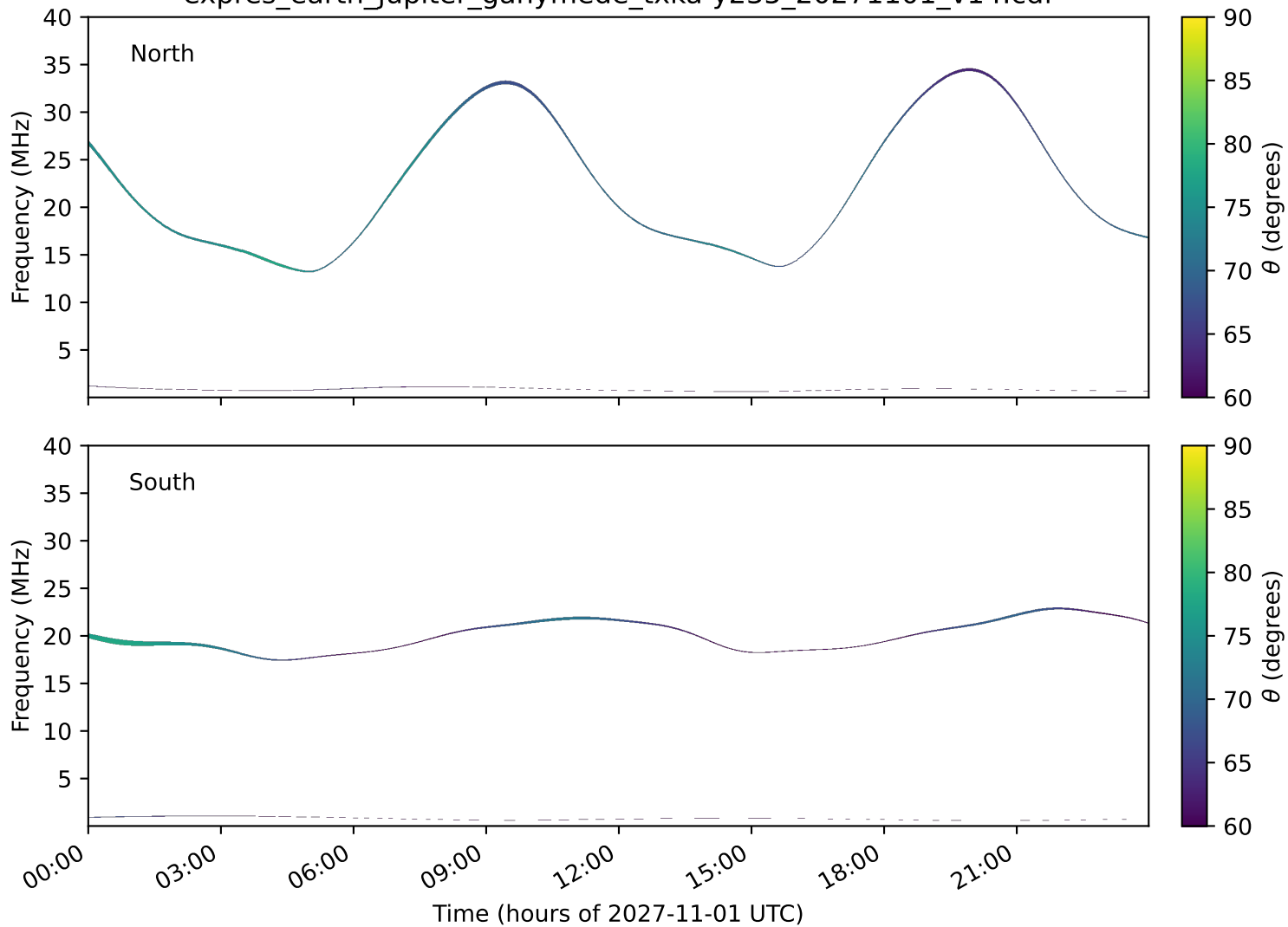
expres_earth_jupiter_ganymede_txka-y235_20271101_v14.cdf
