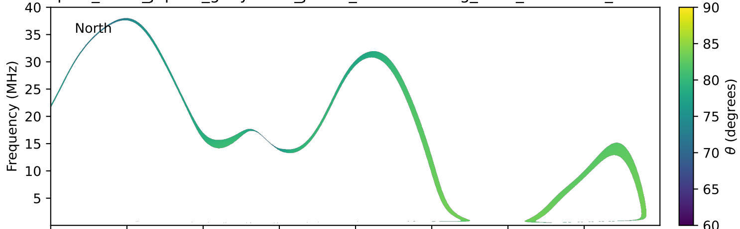
expres_earth_jupiter_ganymede_jrm33_lossc-wid1deg_3kev_20271127_v11.cdf
