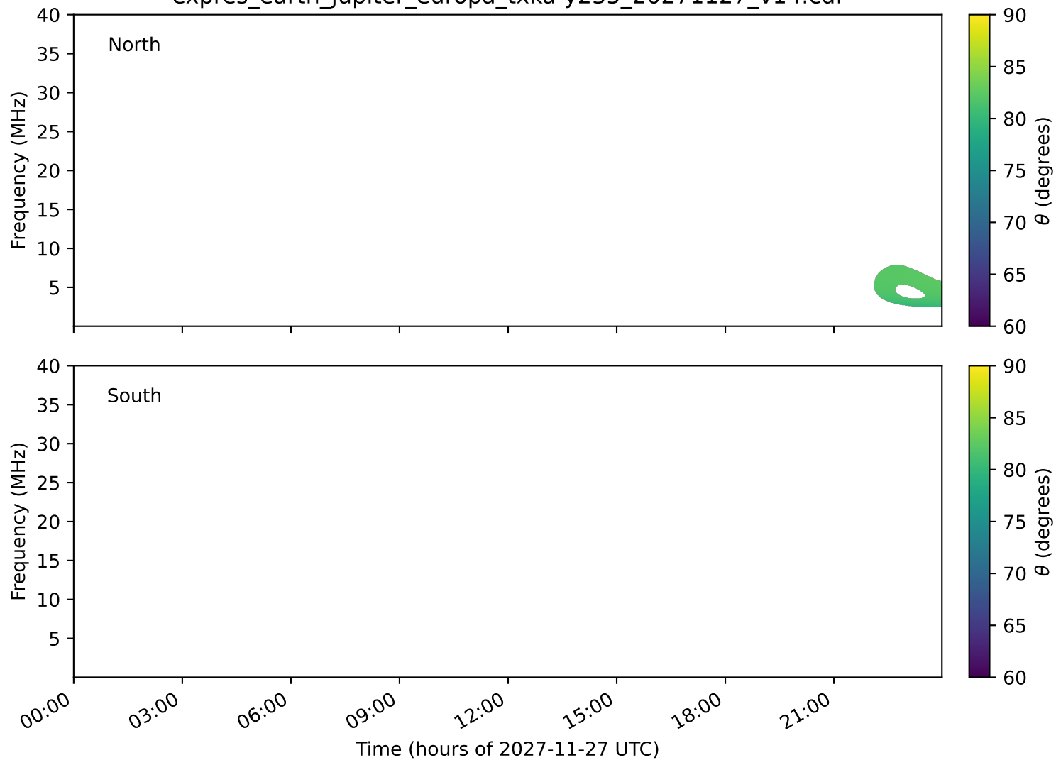
expres_earth_jupiter_europa_txka-y235_20271127_v14.cdf
