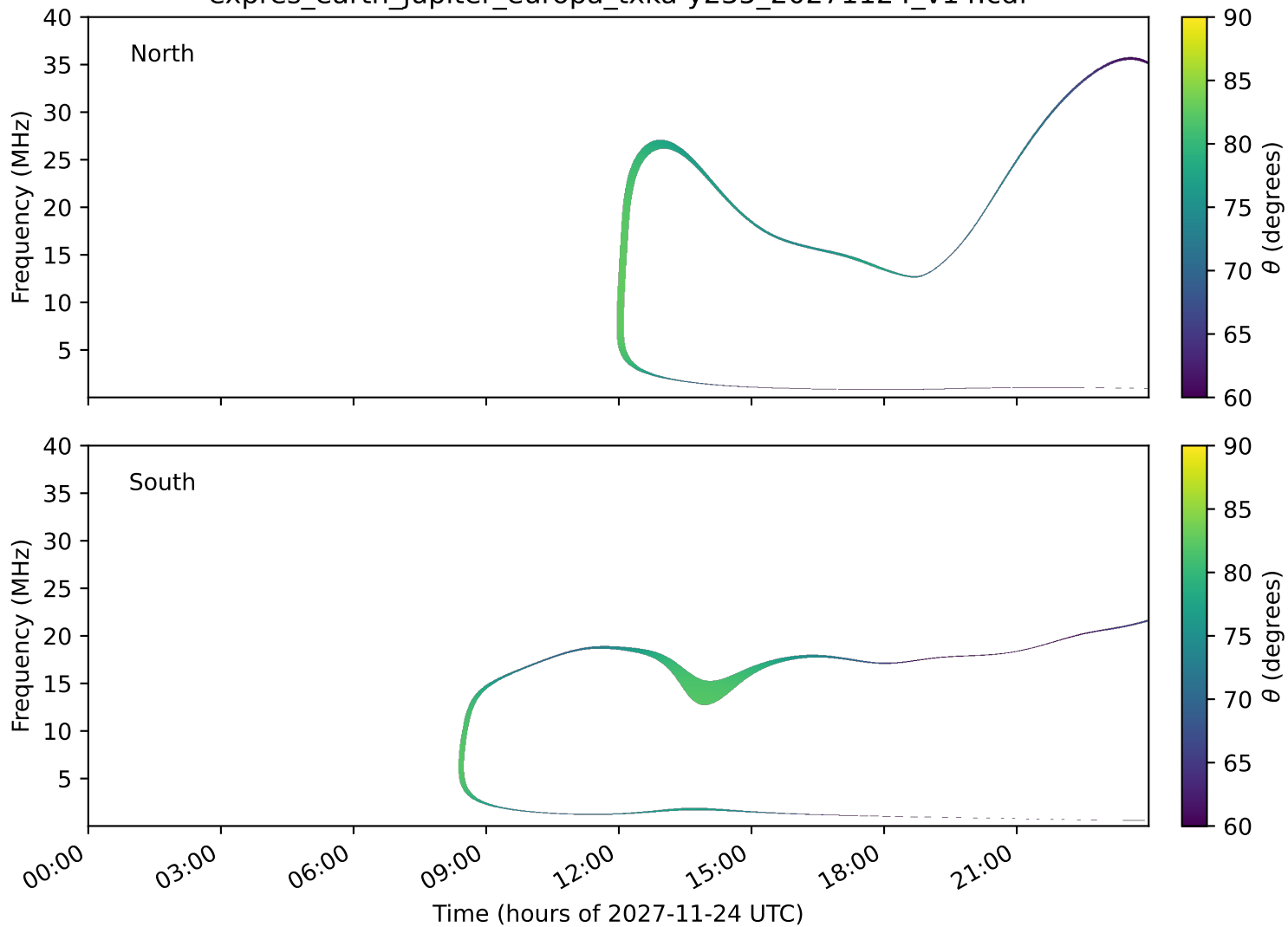
expres_earth_jupiter_europa_txka-y235_20271124_v14.cdf
