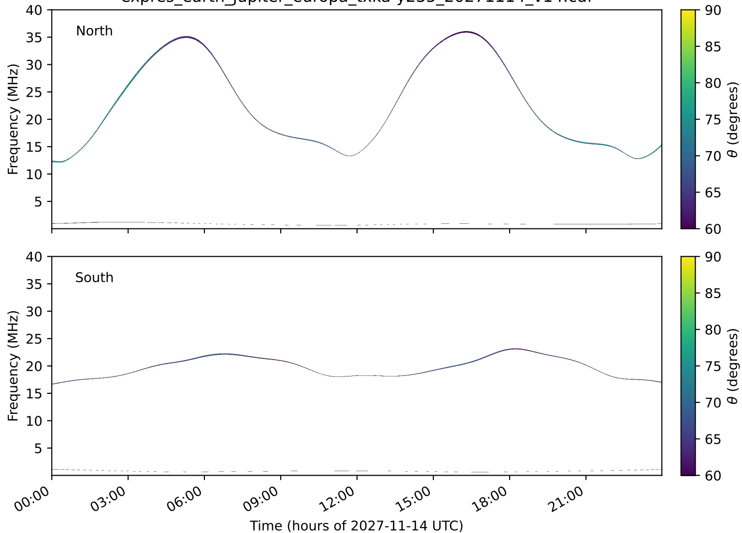
expres_earth_jupiter_europa_txka-y235_20271114_v14.cdf
