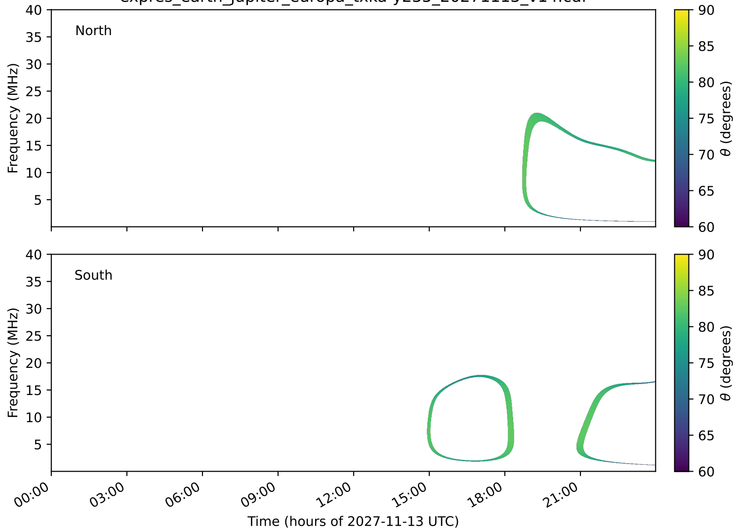
expres_earth_jupiter_europa_txka-y235_20271113_v14.cdf
