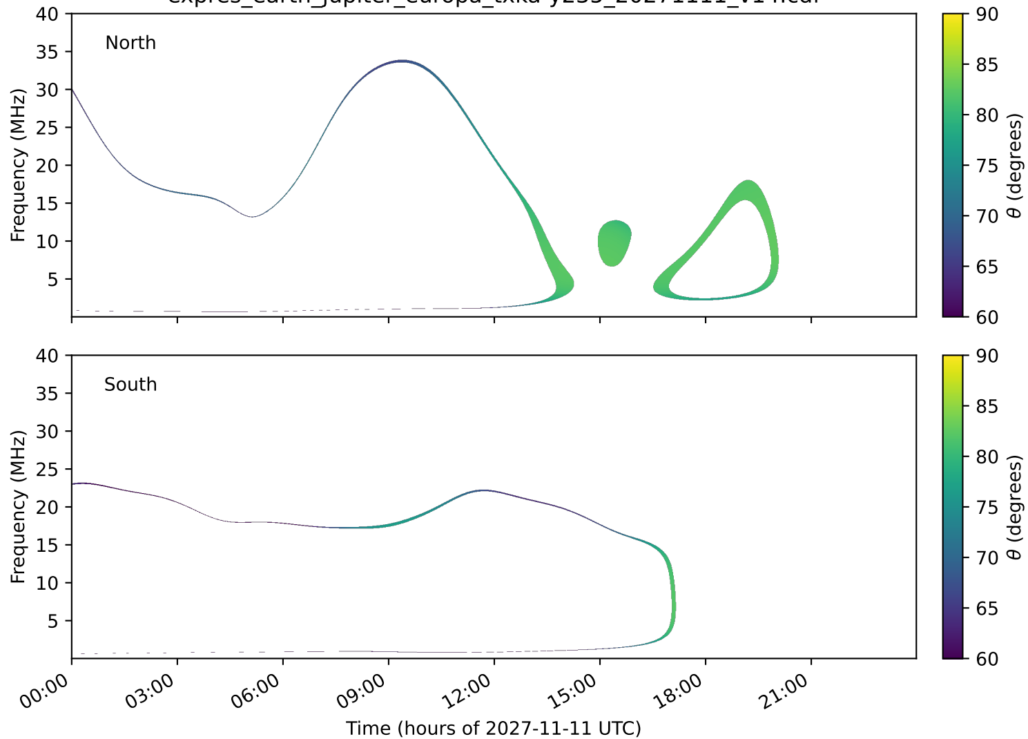
expres_earth_jupiter_europa_txka-y235_20271111_v14.cdf
