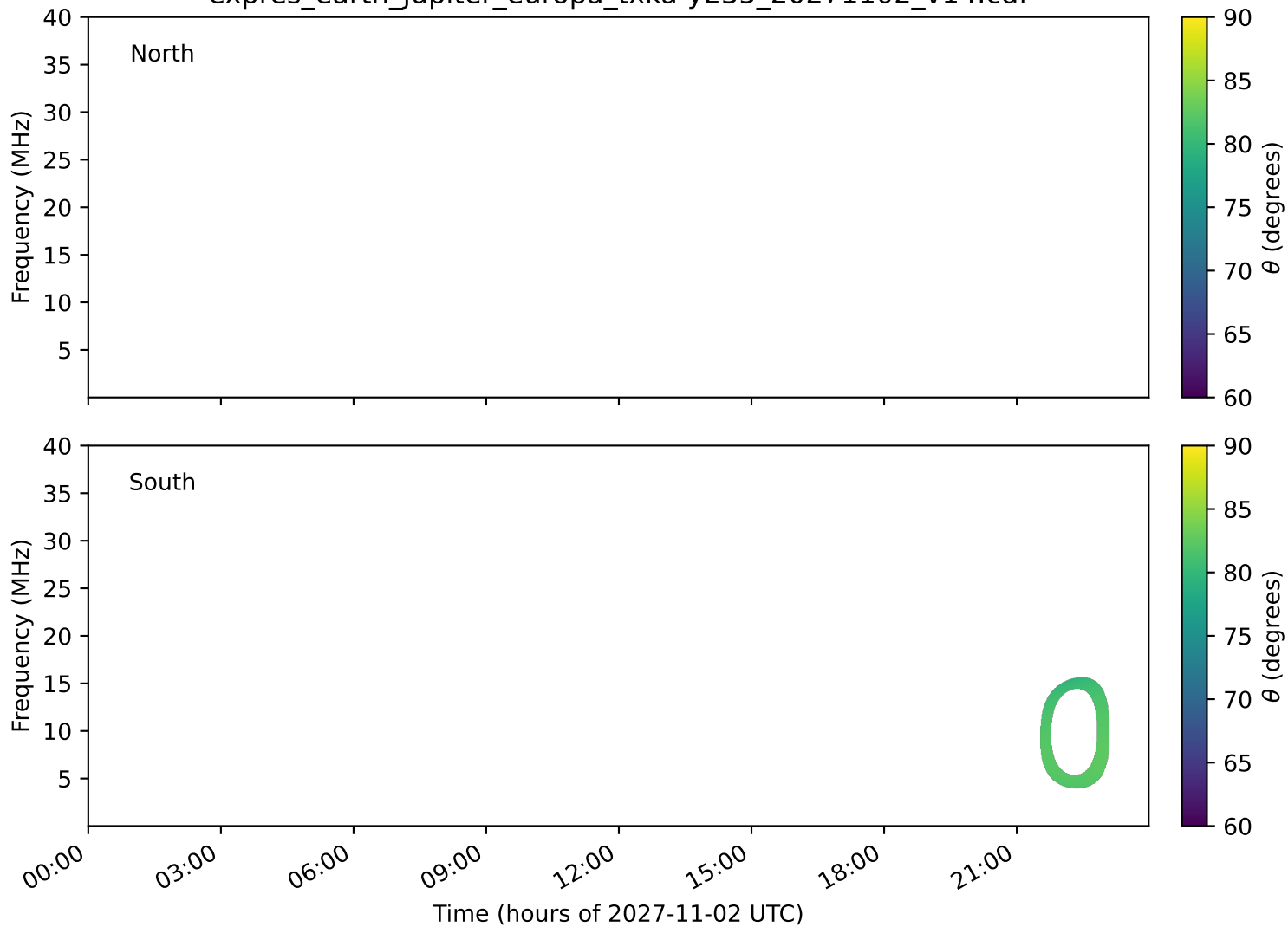
expres_earth_jupiter_europa_txka-y235_20271102_v14.cdf
