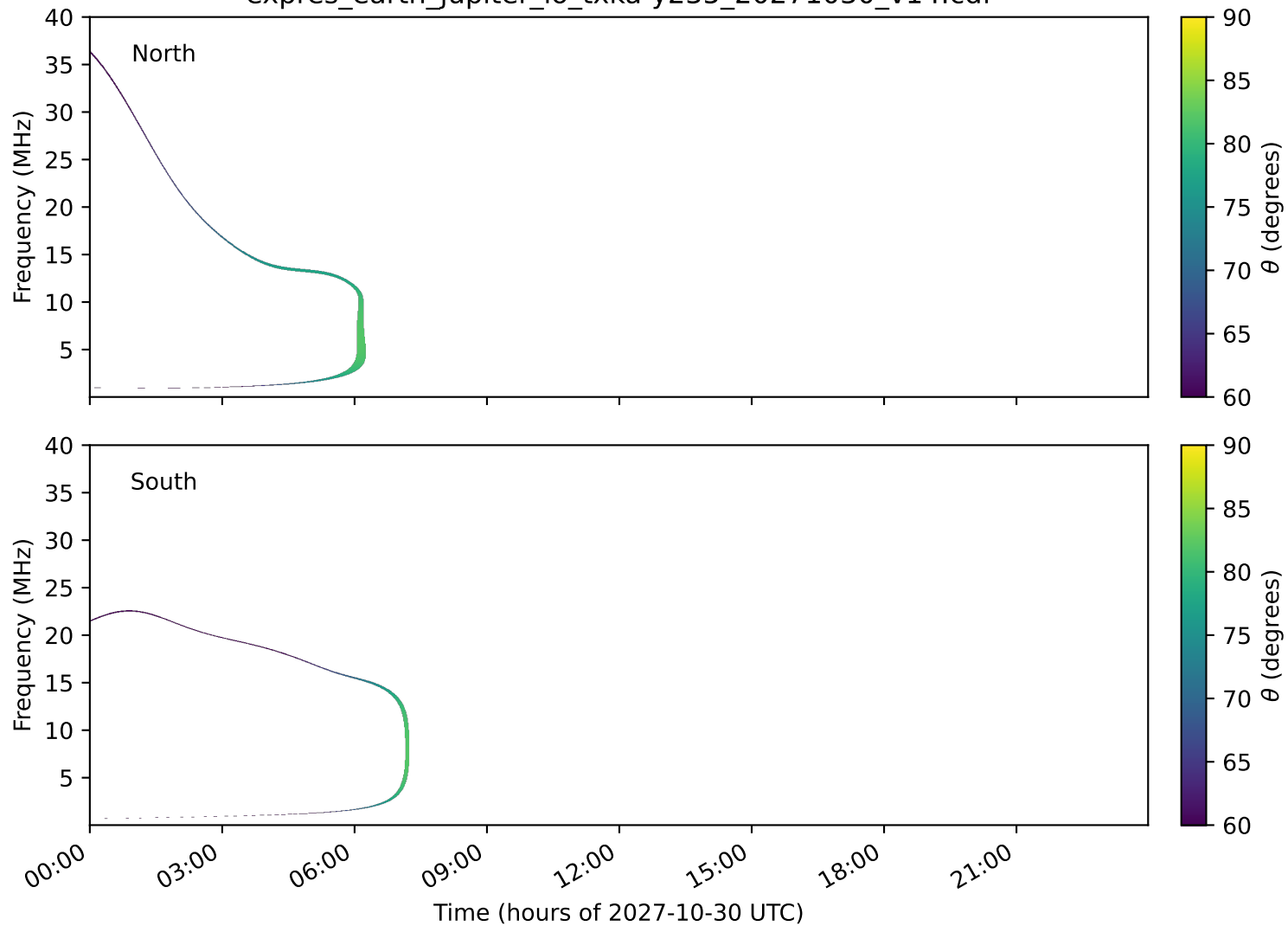
expres_earth_jupiter_io_txka-y235_20271030_v14.cdf
