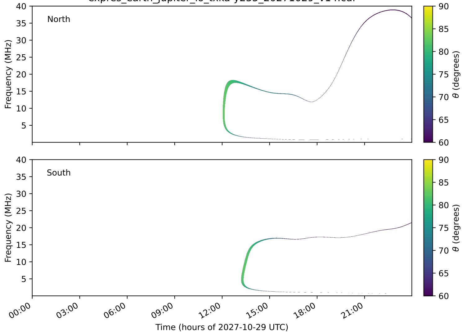
expres_earth_jupiter_io_txka-y235_20271029_v14.cdf
