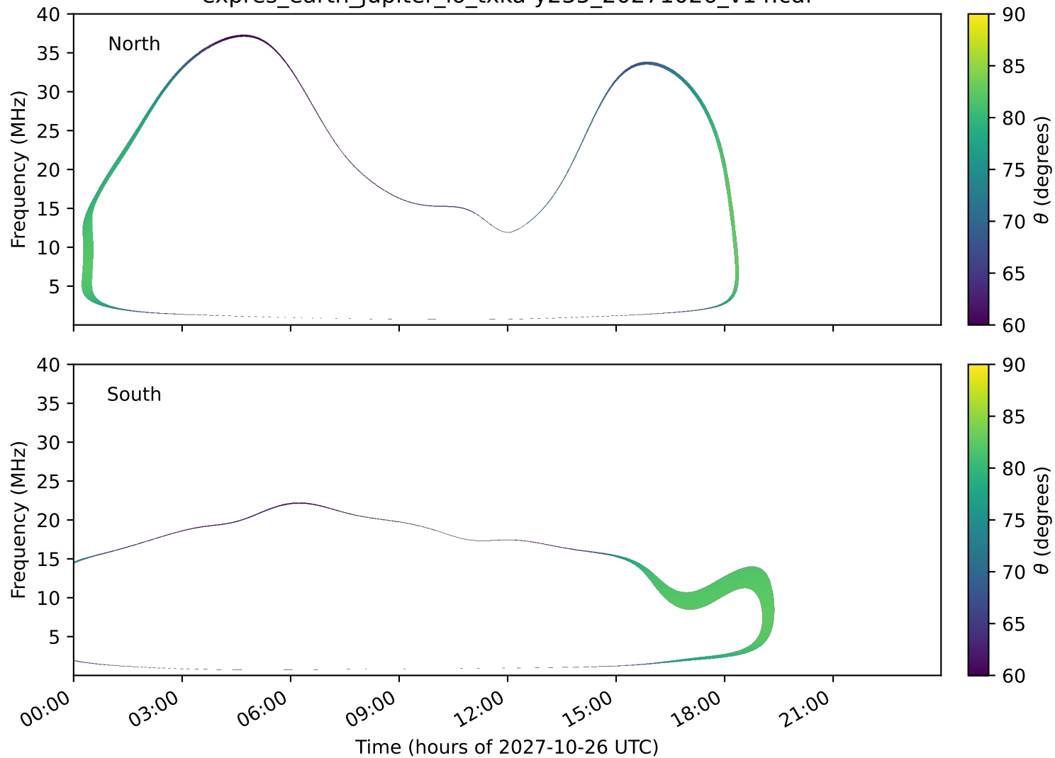
expres_earth_jupiter_io_txka-y235_20271026_v14.cdf
