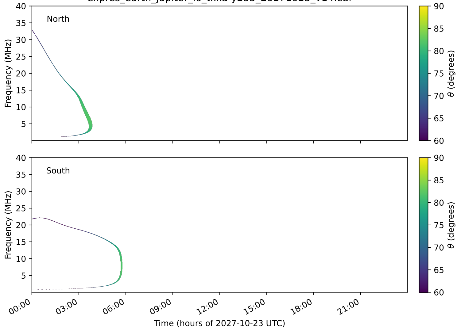
expres_earth_jupiter_io_txka-y235_20271023_v14.cdf
