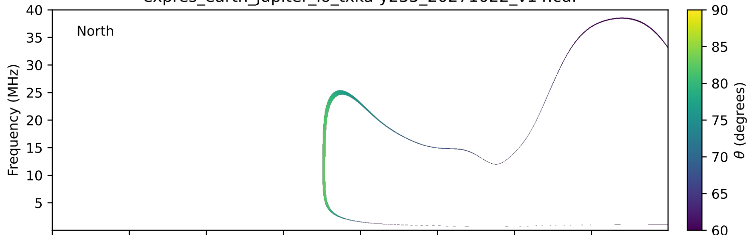
expres_earth_jupiter_io_txka-y235_20271022_v14.cdf
