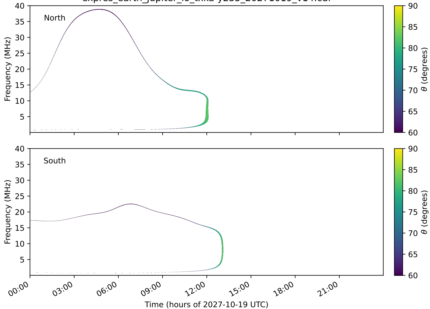
expres_earth_jupiter_io_txka-y235_20271019_v14.cdf
