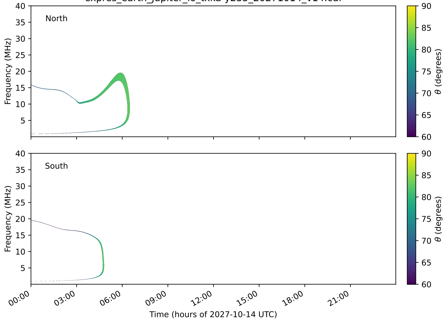
expres_earth_jupiter_io_txka-y235_20271014_v14.cdf
