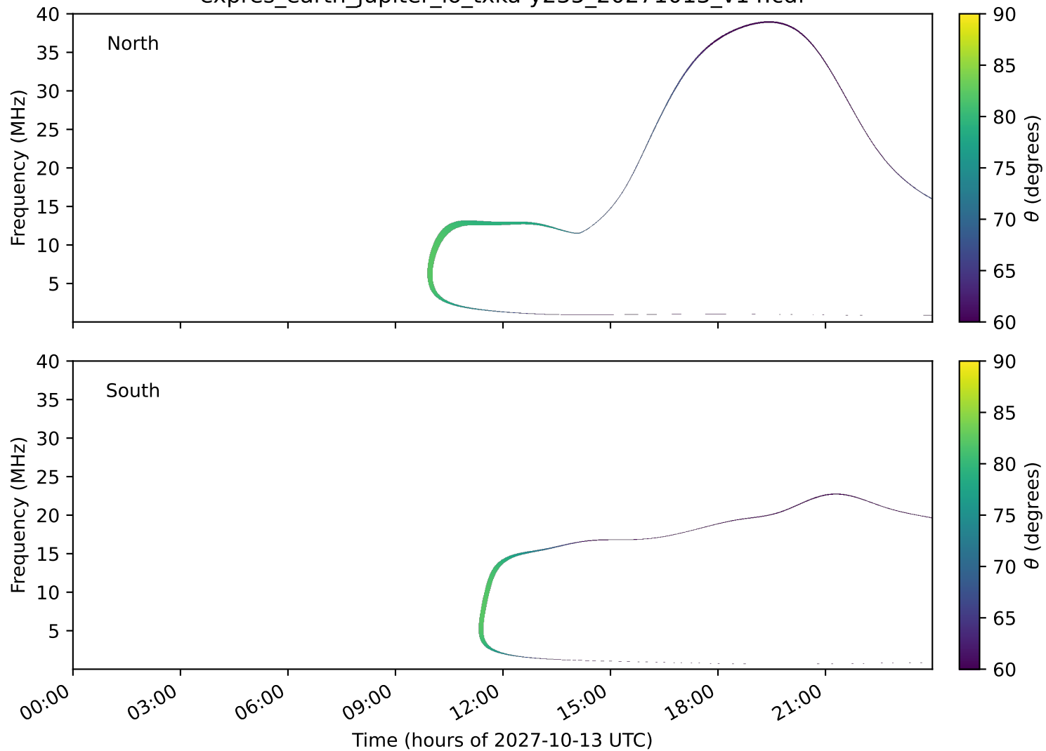
expres_earth_jupiter_io_txka-y235_20271013_v14.cdf
