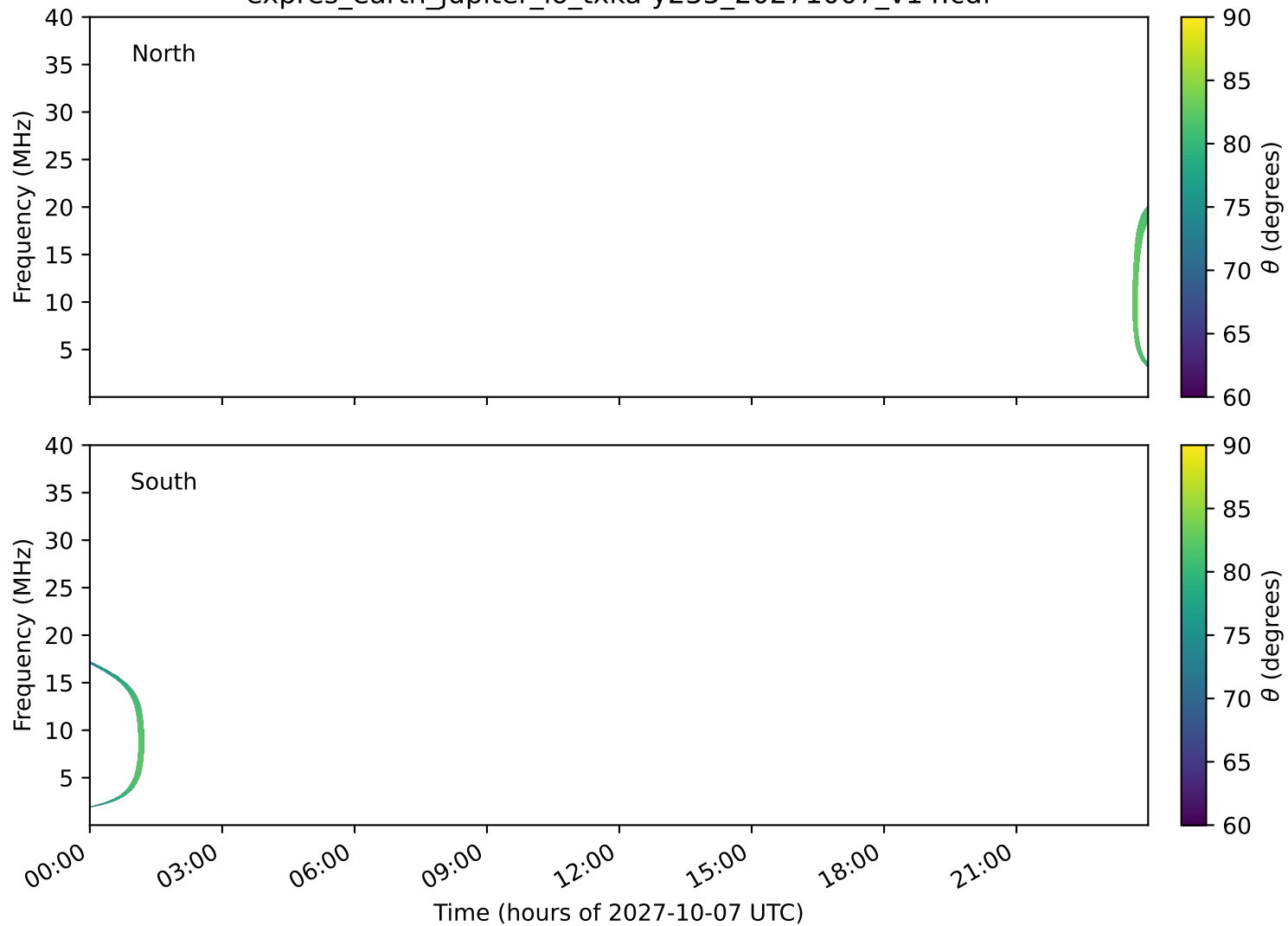
expres_earth_jupiter_io_txka-y235_20271007_v14.cdf
