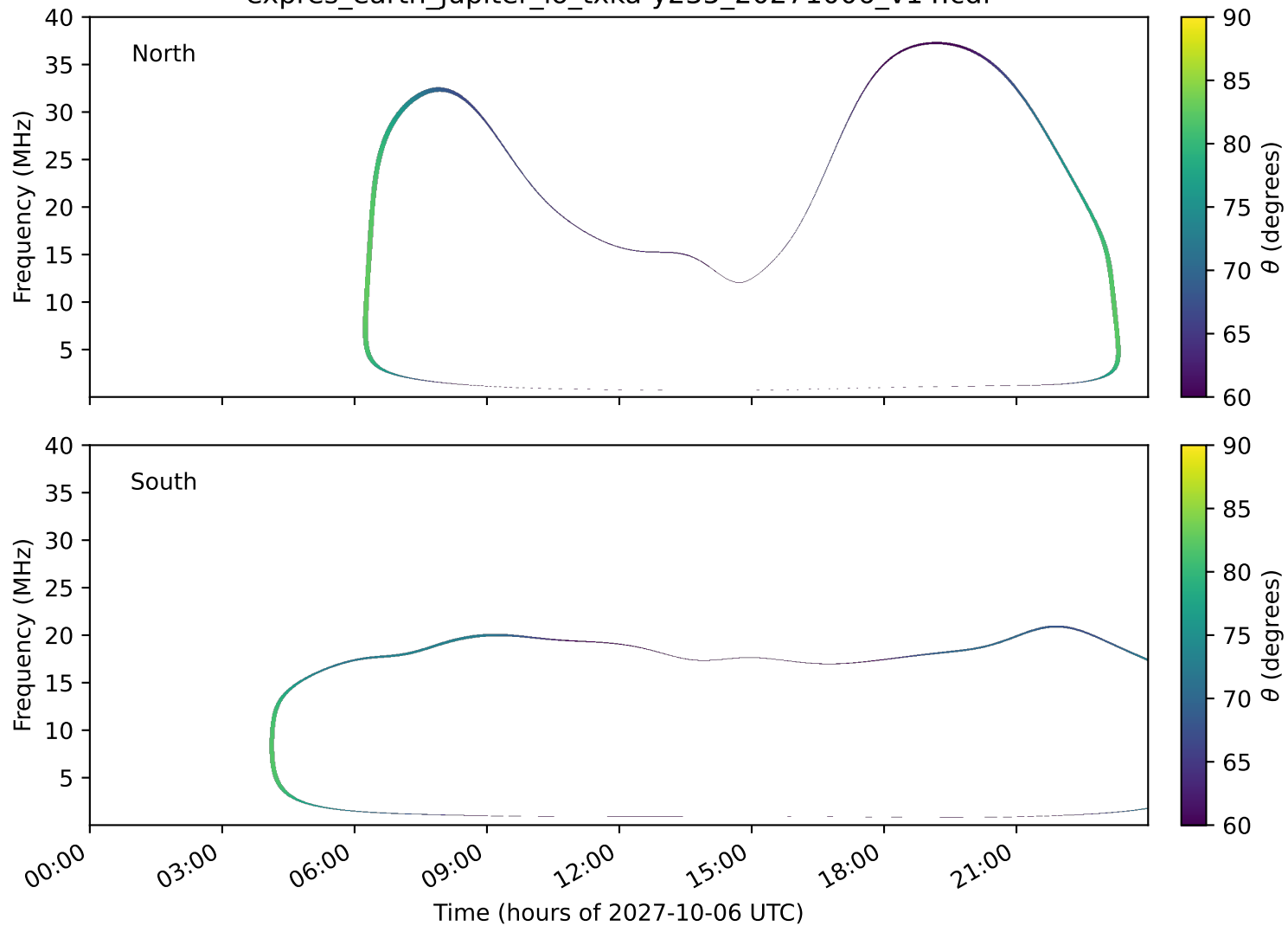
expres_earth_jupiter_io_txka-y235_20271006_v14.cdf
