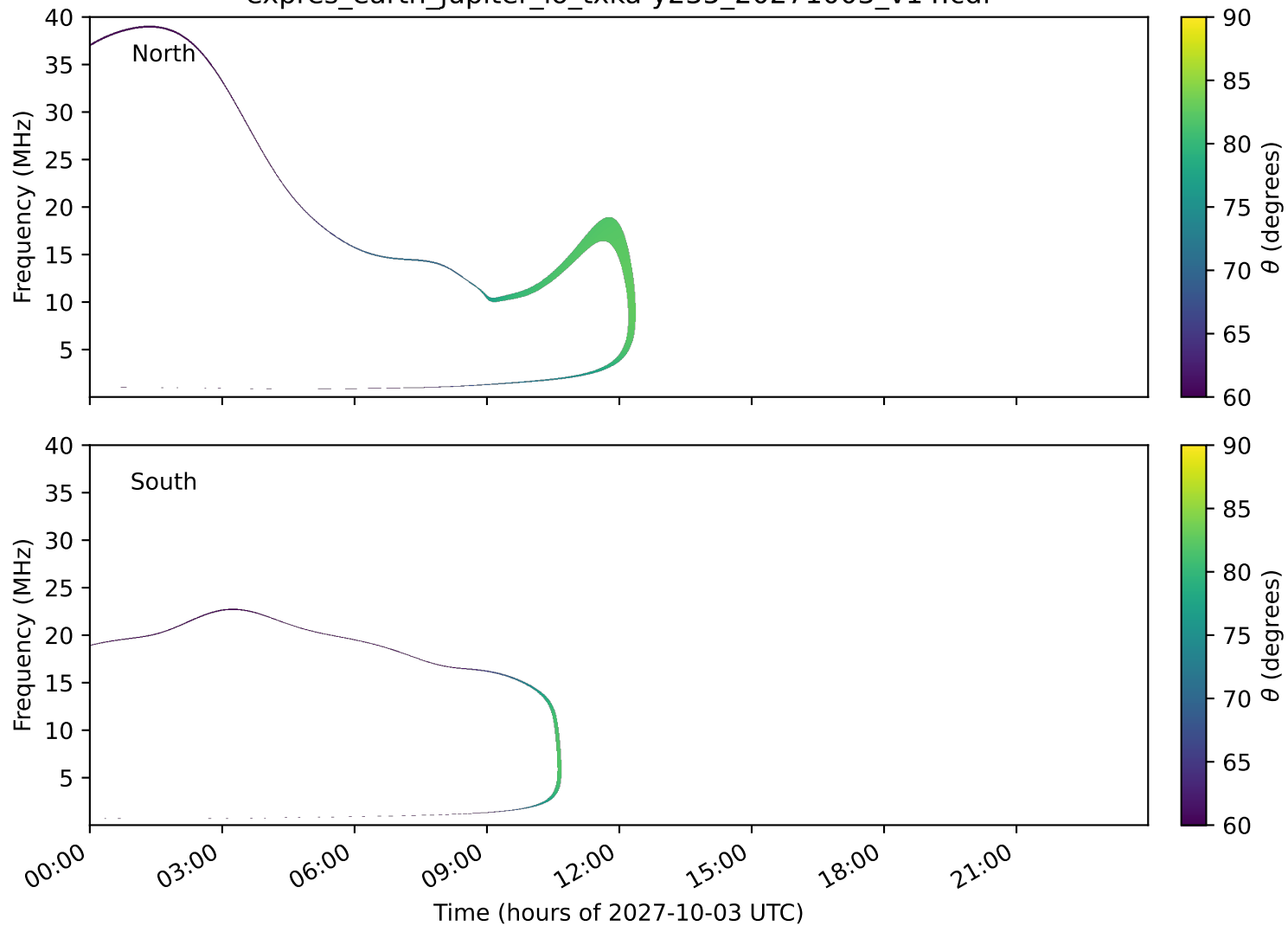
expres_earth_jupiter_io_txka-y235_20271003_v14.cdf
