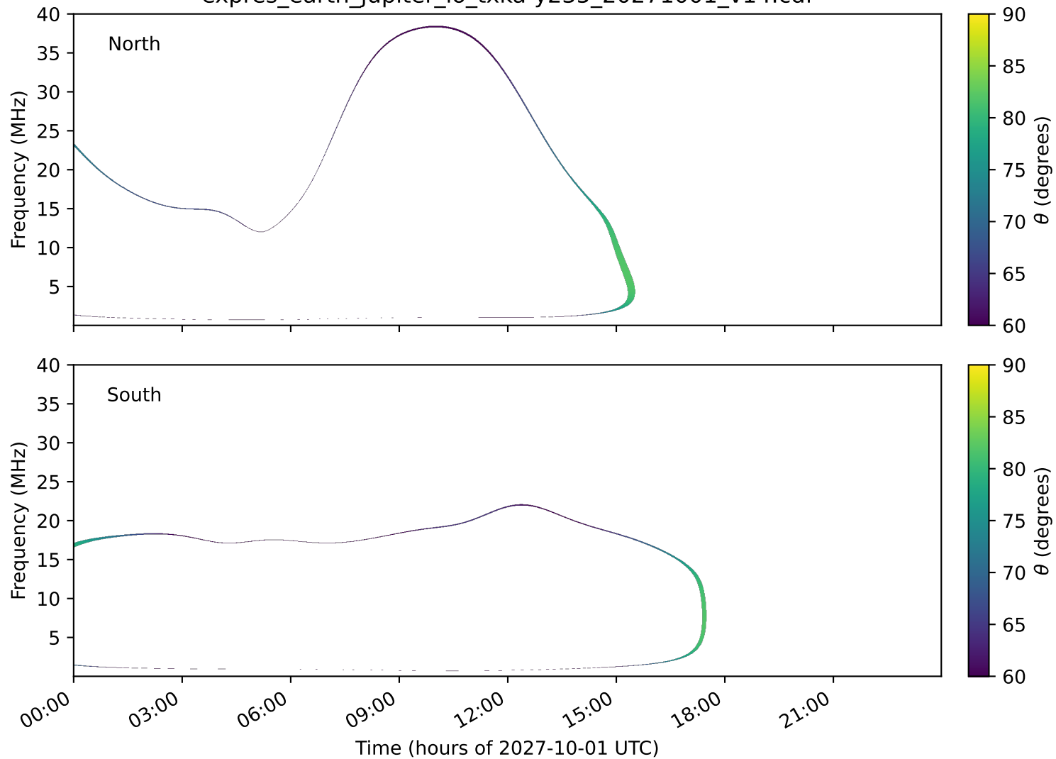
expres_earth_jupiter_io_txka-y235_20271001_v14.cdf
