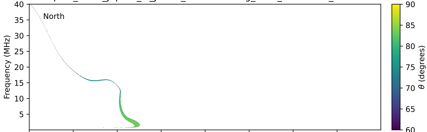
expres_earth_jupiter_io_jrm33_lossc-wid1deg_3kev_20271030_v11.cdf
