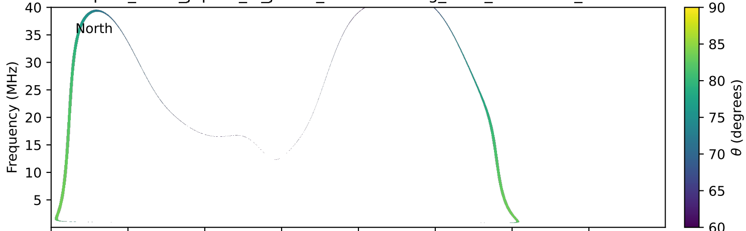
expres_earth_jupiter_io_jrm33_lossc-wid1deg_3kev_20271017_v11.cdf
