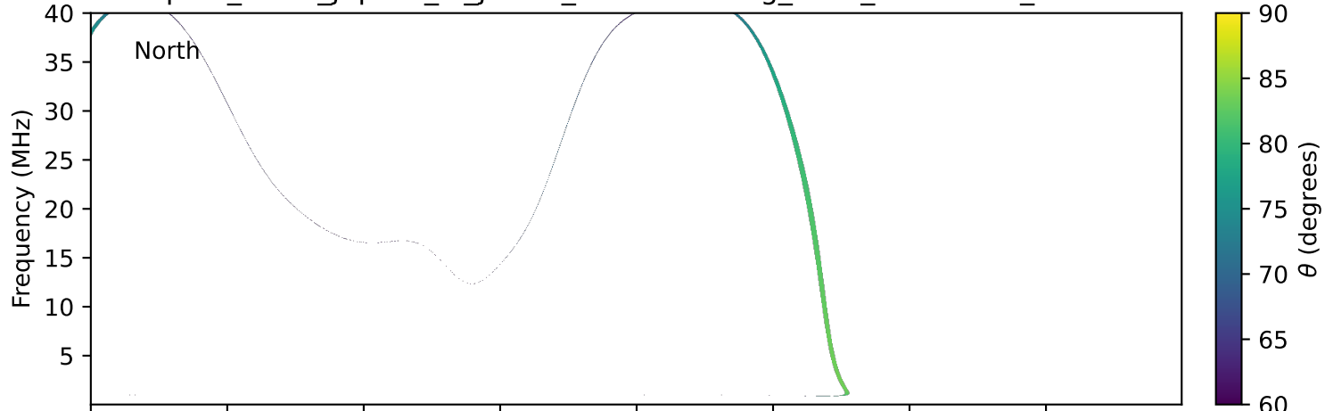
expres_earth_jupiter_io_jrm33_lossc-wid1deg_3kev_20271010_v11.cdf
