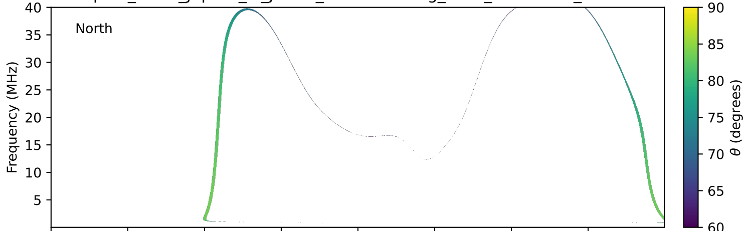
expres_earth_jupiter_io_jrm33_lossc-wid1deg_3kev_20271006_v11.cdf
