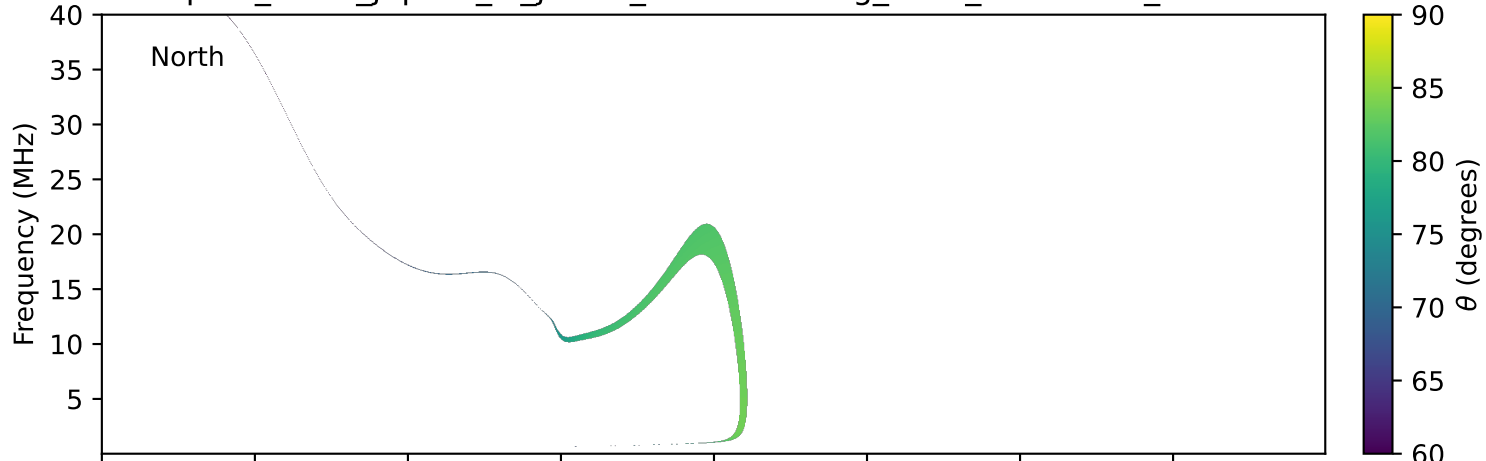
expres_earth_jupiter_io_jrm33_lossc-wid1deg_3kev_20271003_v11.cdf
