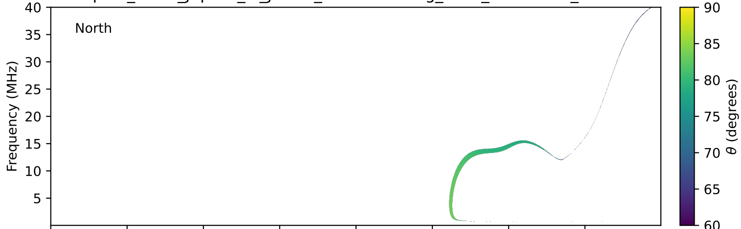
expres_earth_jupiter_io_jrm33_lossc-wid1deg_3kev_20271002_v11.cdf
