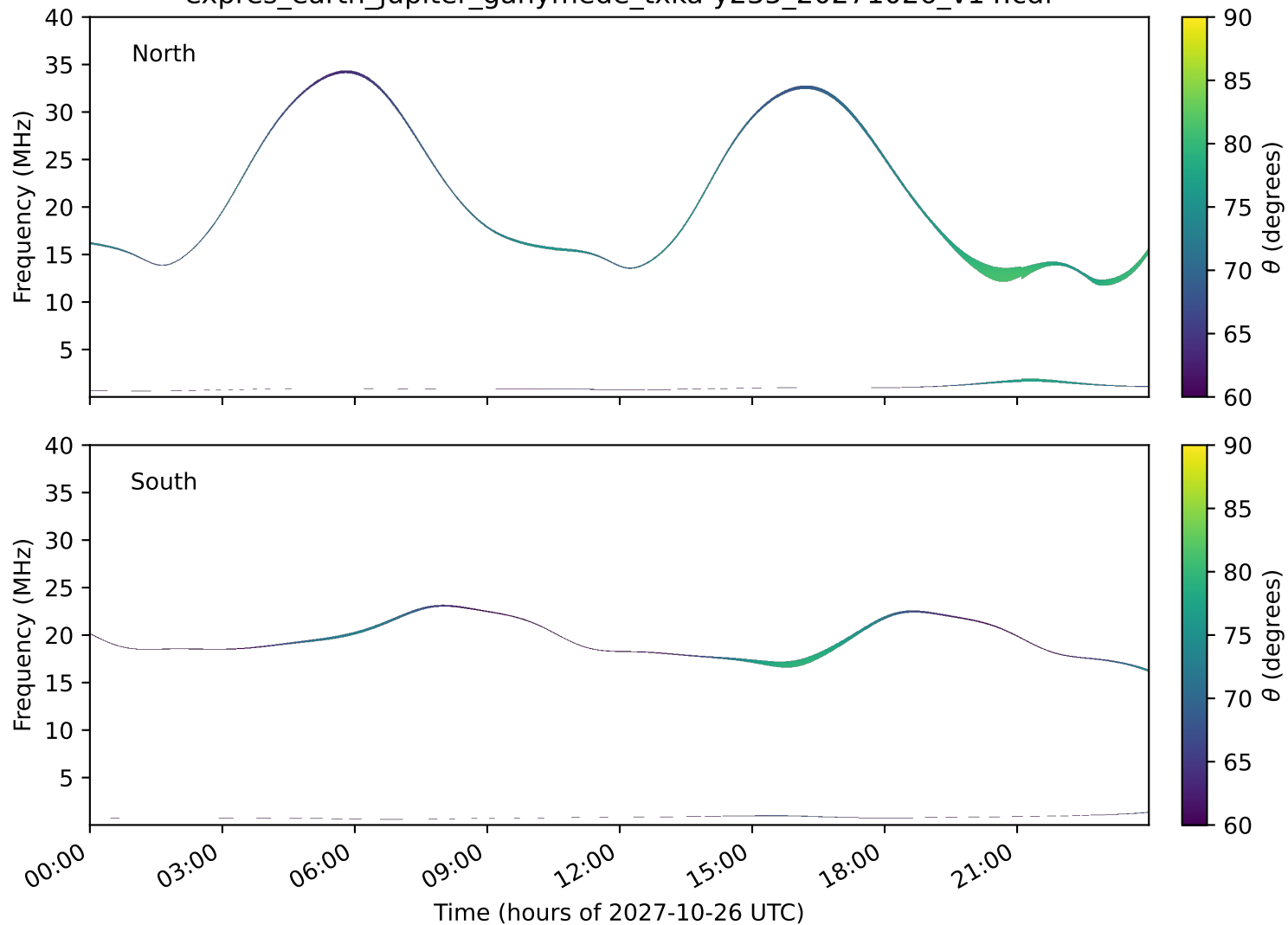
expres_earth_jupiter_ganymede_txka-y235_20271026_v14.cdf
