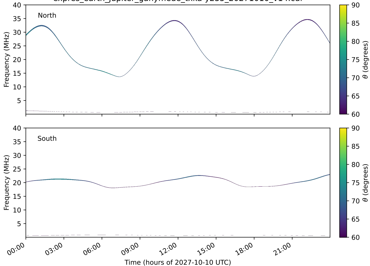
expres_earth_jupiter_ganymede_txka-y235_20271010_v14.cdf
