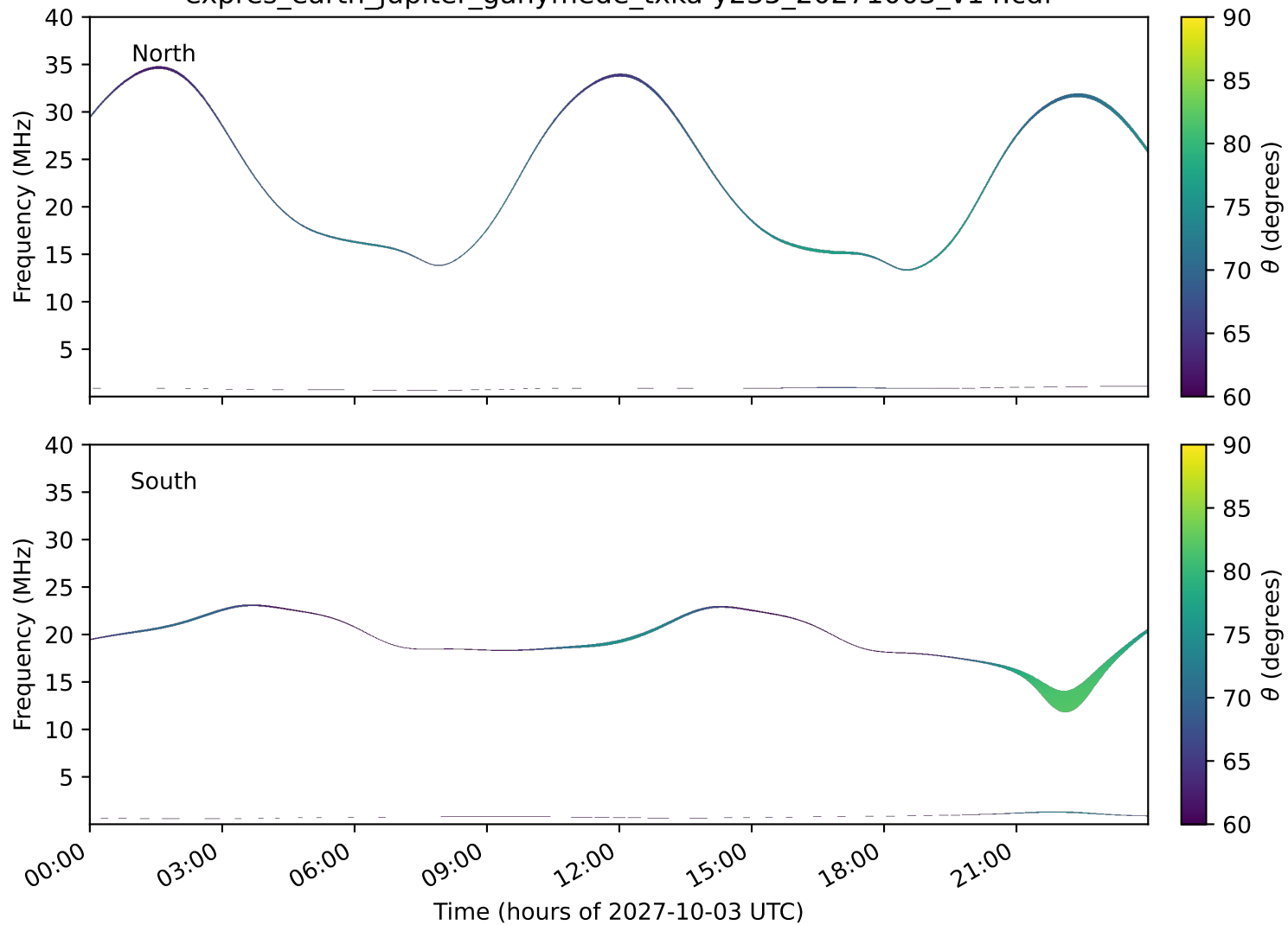
expres_earth_jupiter_ganymede_txka-y235_20271003_v14.cdf
