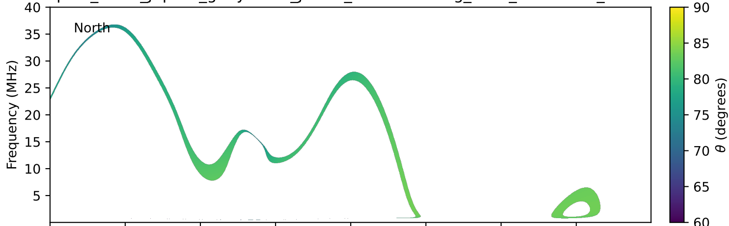
expres_earth_jupiter_ganymede_jrm33_lossc-wid1deg_3kev_20271027_v11.cdf
