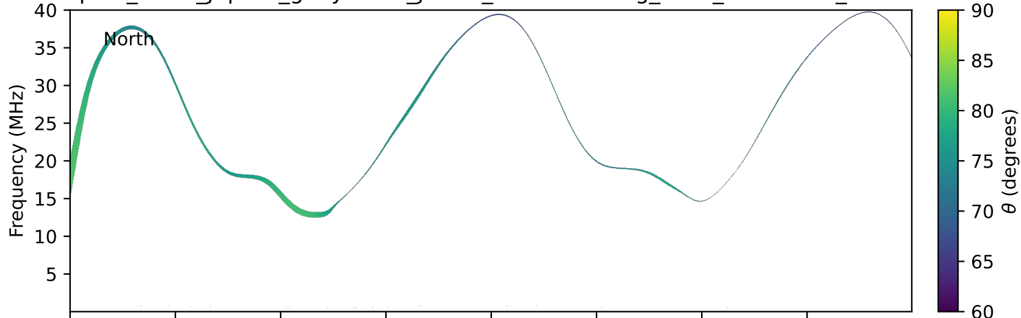
expres_earth_jupiter_ganymede_jrm33_lossc-wid1deg_3kev_20271017_v11.cdf
