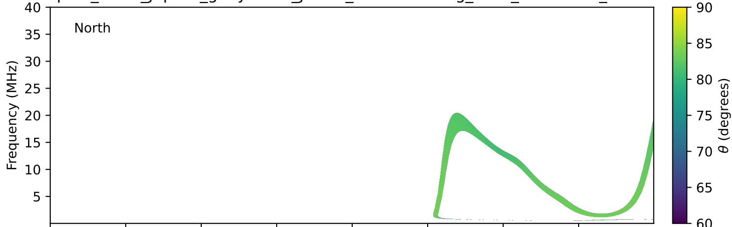
expres_earth_jupiter_ganymede_jrm33_lossc-wid1deg_3kev_20271016_v11.cdf
