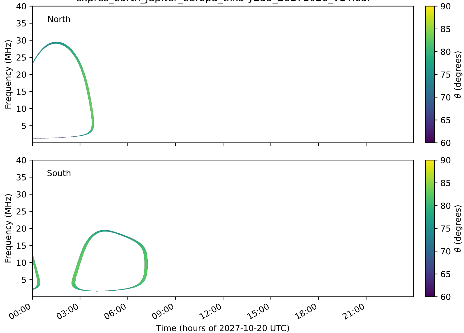
expres_earth_jupiter_europa_txka-y235_20271020_v14.cdf
