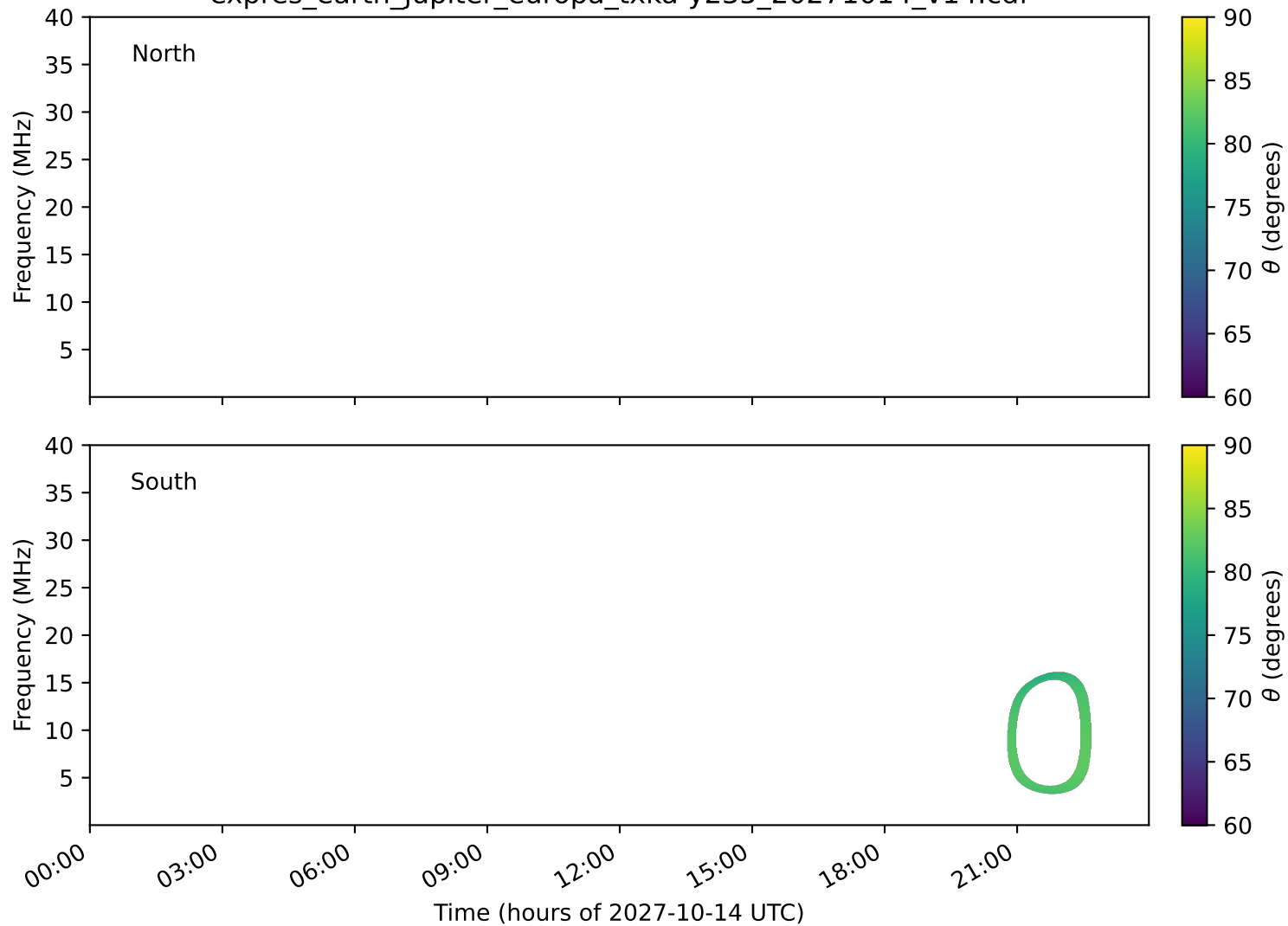
expres_earth_jupiter_europa_txka-y235_20271014_v14.cdf
