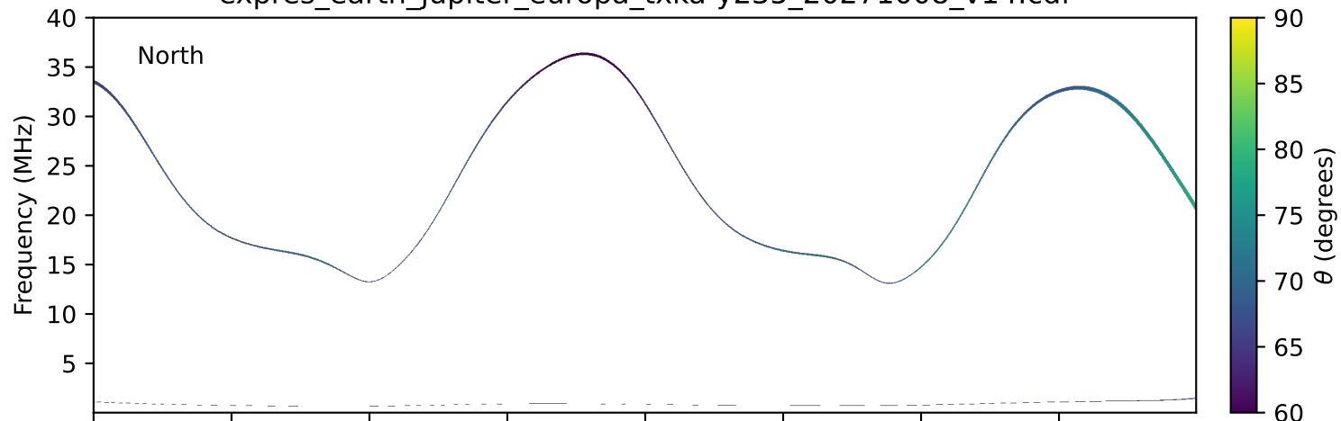
expres_earth_jupiter_europa_txka-y235_20271008_v14.cdf
