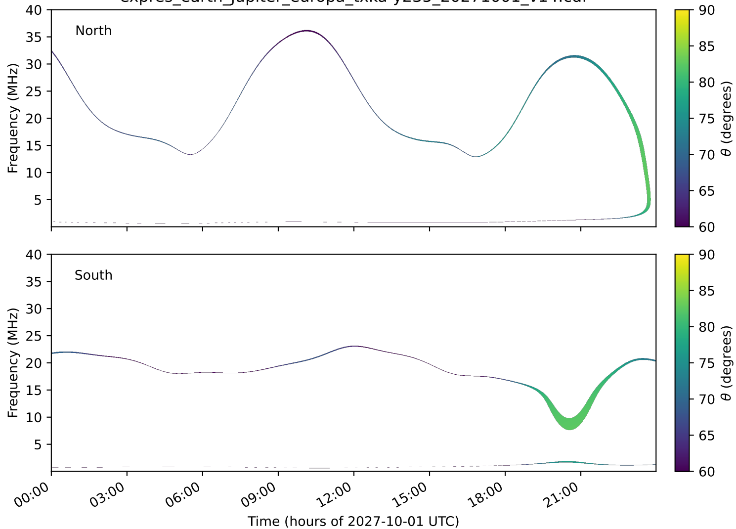
expres_earth_jupiter_europa_txka-y235_20271001_v14.cdf
