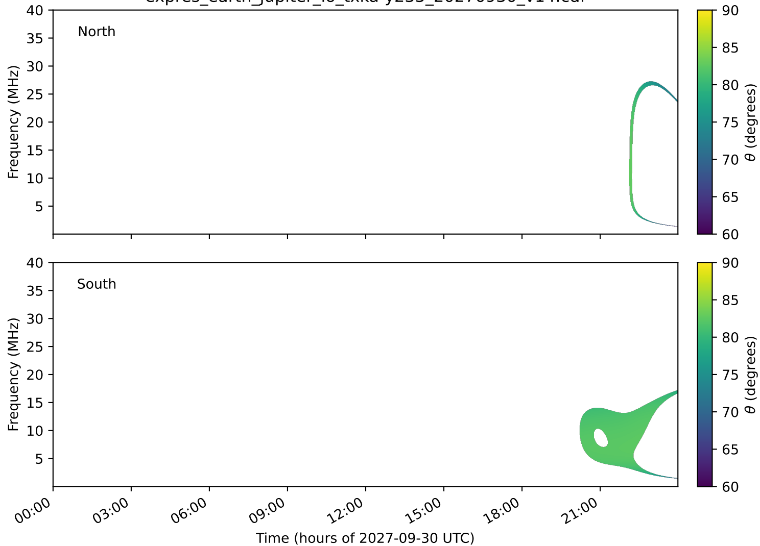
expres_earth_jupiter_io_txka-y235_20270930_v14.cdf
