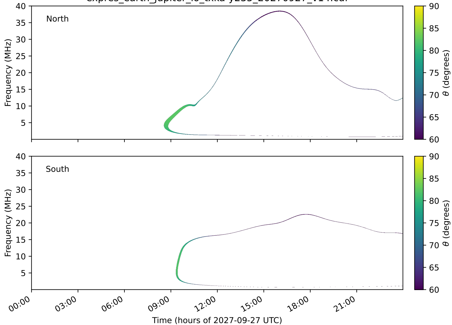
expres_earth_jupiter_io_txka-y235_20270927_v14.cdf
